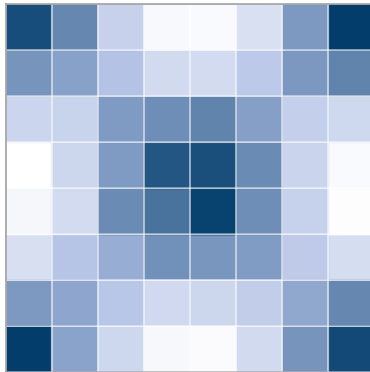
PIC: deposit to 8x8 grid
