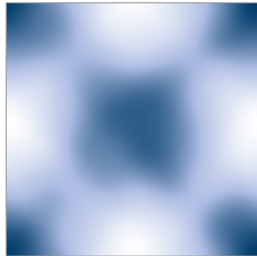
PIF: 8x8 Fourier modes, no grid
