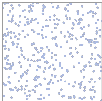
400 distinct particles
