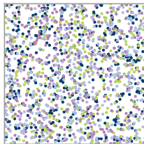
1600 distinct particles
