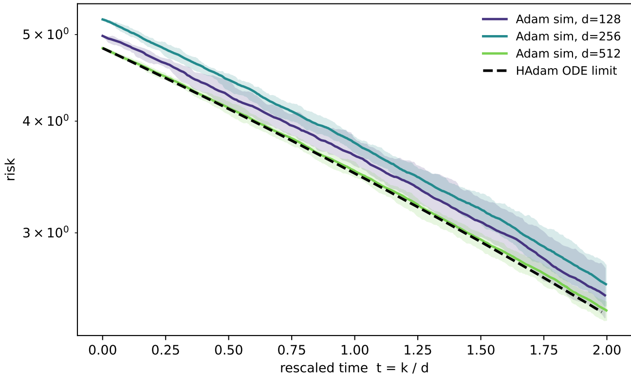
Adam: finite-d simulator \rightarrow HAdam limit (linreg, \beta_1=0.1 , \beta_2=0.1 )
