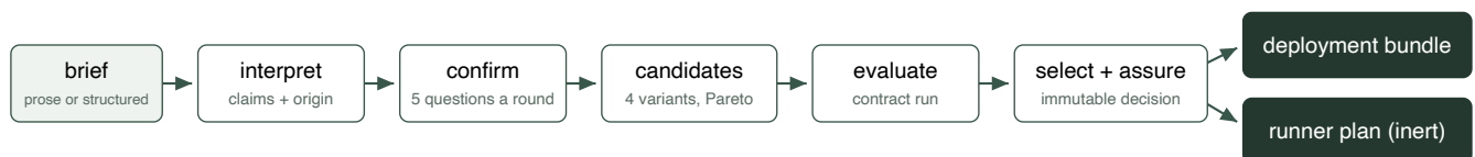
Figure 1 — the pipeline. The compiled plan is inert: executing anything requires the separate signing, approval and runner verification described in chapter 6.
