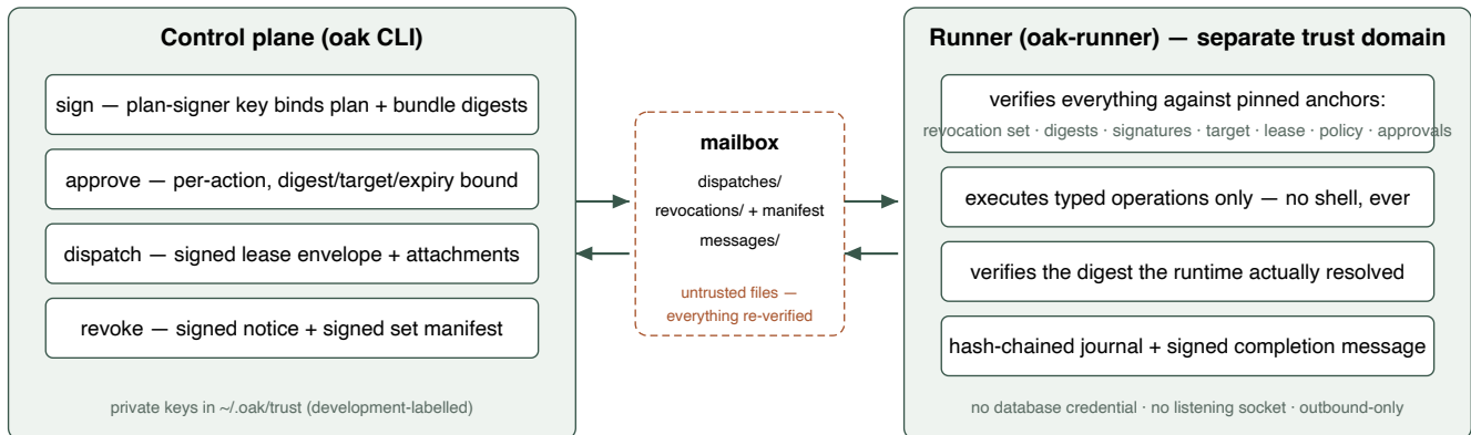
Figure 3 — two trust domains, one untrusted mailbox. A tampered mailbox file is an expected adversarial case: the runner recomputes and re-verifies everything from pinned keys, and any failure is a denial with a stable code, published back as a signed message.
