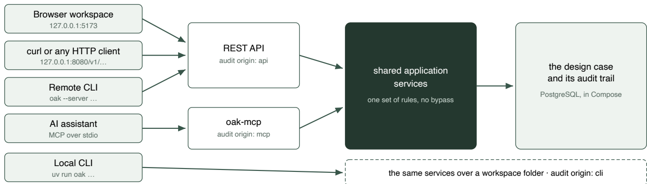
Figure 2 — five ways in, one set of rules. The browser and the remote CLI are clients of the REST API, so their steps are recorded as api . An export moves a case between a workspace folder and the server.
