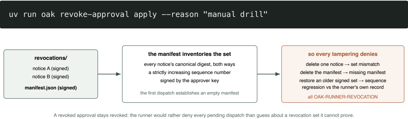
Figure 4 — the revocation channel. Notices and their signed set manifest; the runner records the highest manifest sequence it has seen in its own home directory.
