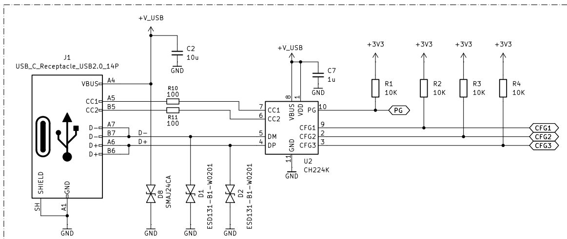
USB-C Connector & PD Controller
