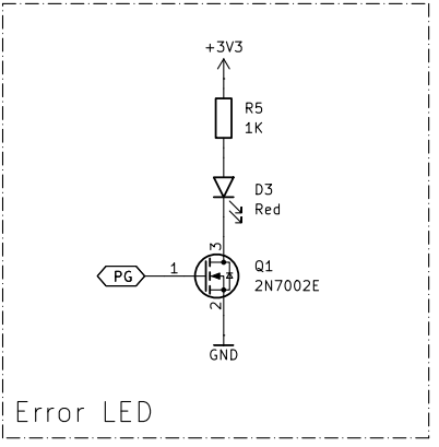
LED voltage indicators
