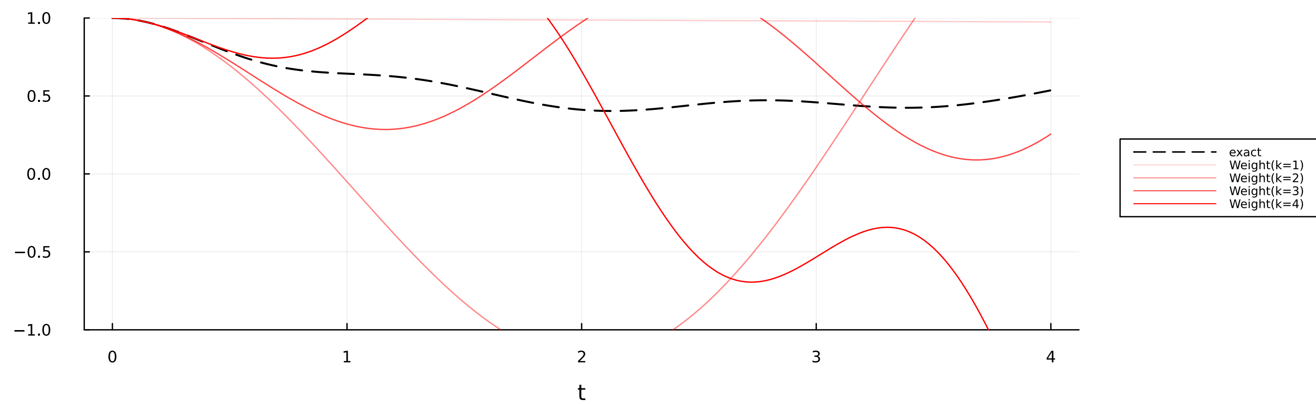
MeanFieldTruncation
