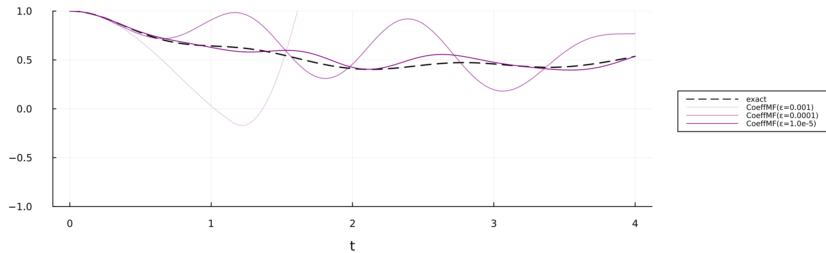
WeightTruncation
