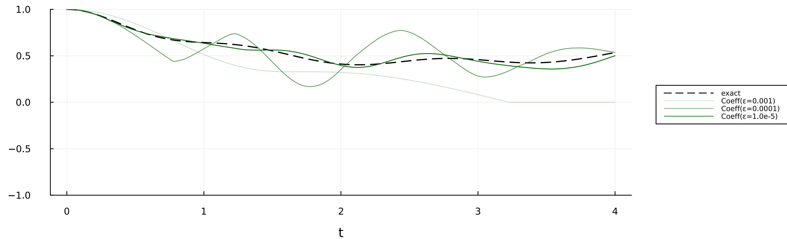
CoeffTruncationMF
