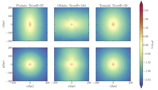
Figure 24. Density contours in the x - z and x - y planes of the prolate, oblate and triaxial halos are shown. The coefficients were computed up to n_{\text{max}} = 20 and the \Gamma = 5 was used to truncate the expansion. For the oblate halo the expansion needs high-order terms to reproduce the density field.
