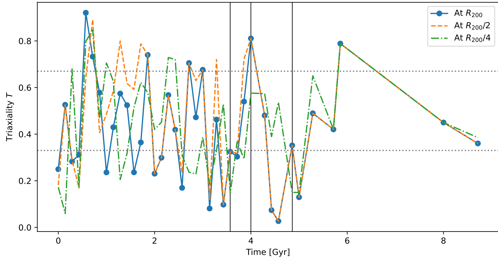
Triaxiality Evolution of M33's DM Halo
