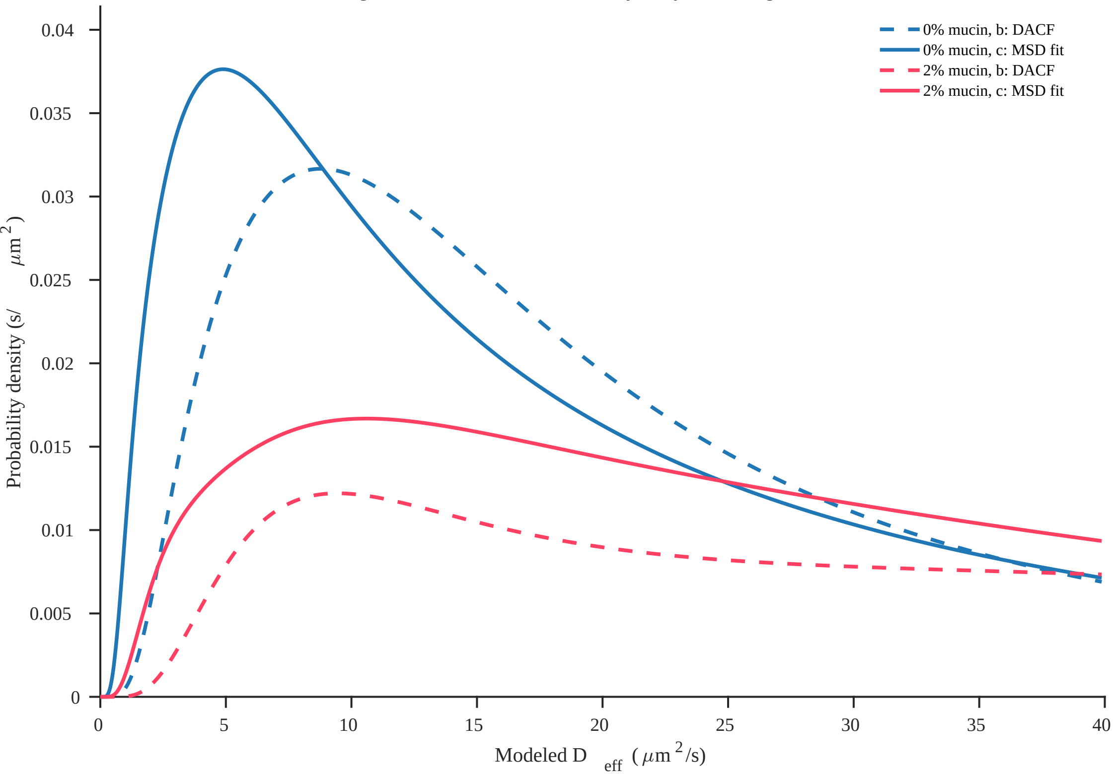
Long-time diffusion after SG3/11 trajectory smoothing
