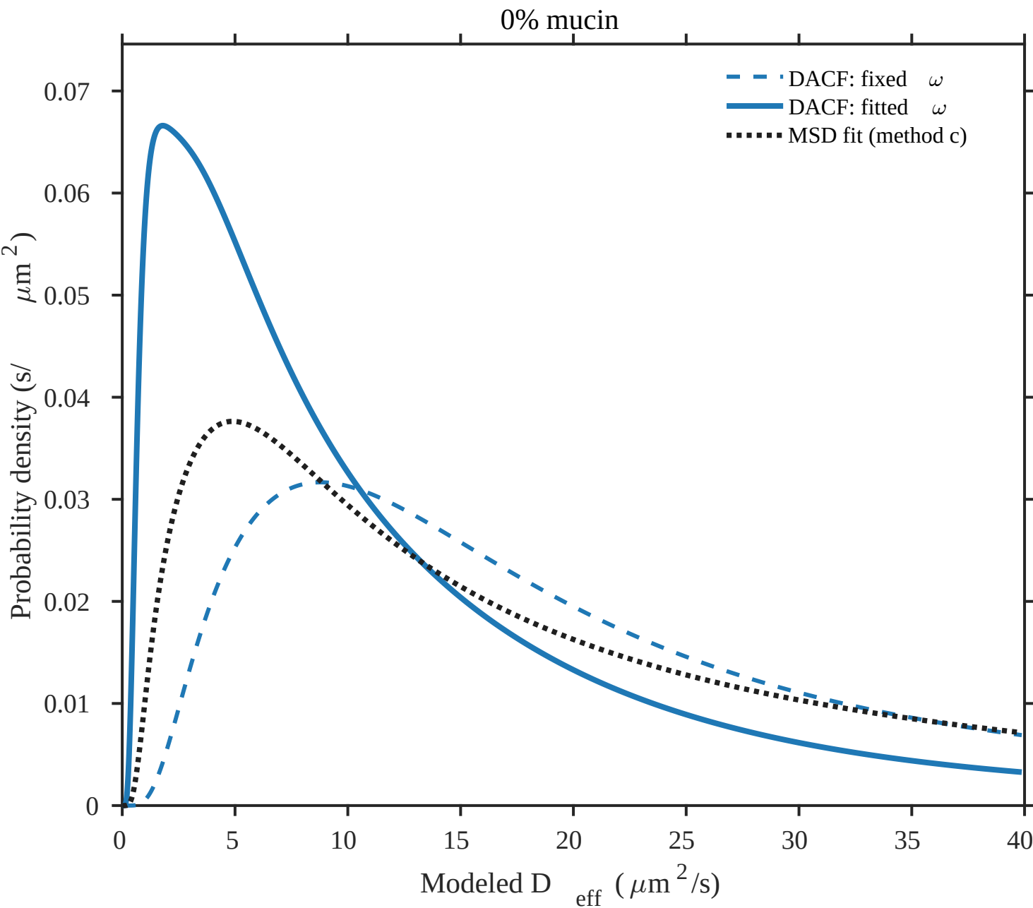
SG3/11 trajectories: jointly fitting D_r and \omega to the DACF
