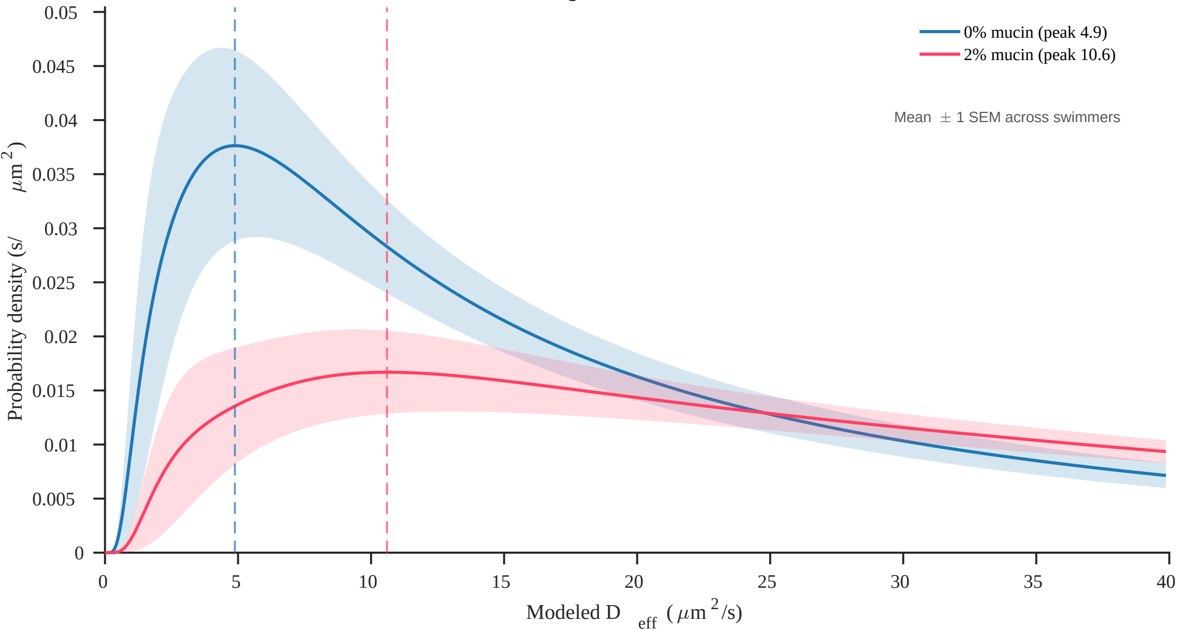
Method c: single-swimmer MSD fits
