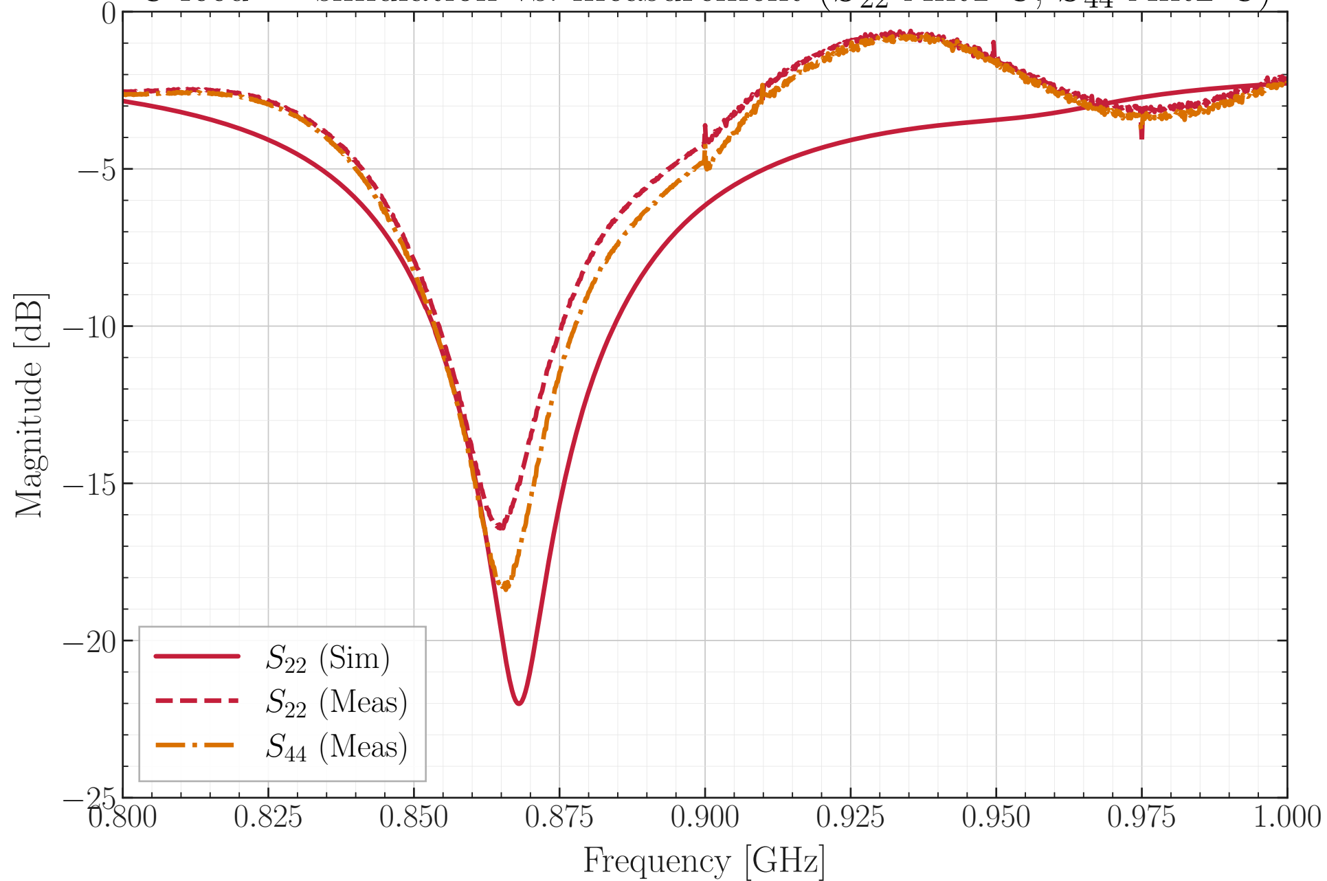
C feed — simulation vs. measurement ( S_{22} Ant1-C, S_{44} Ant2-C)
