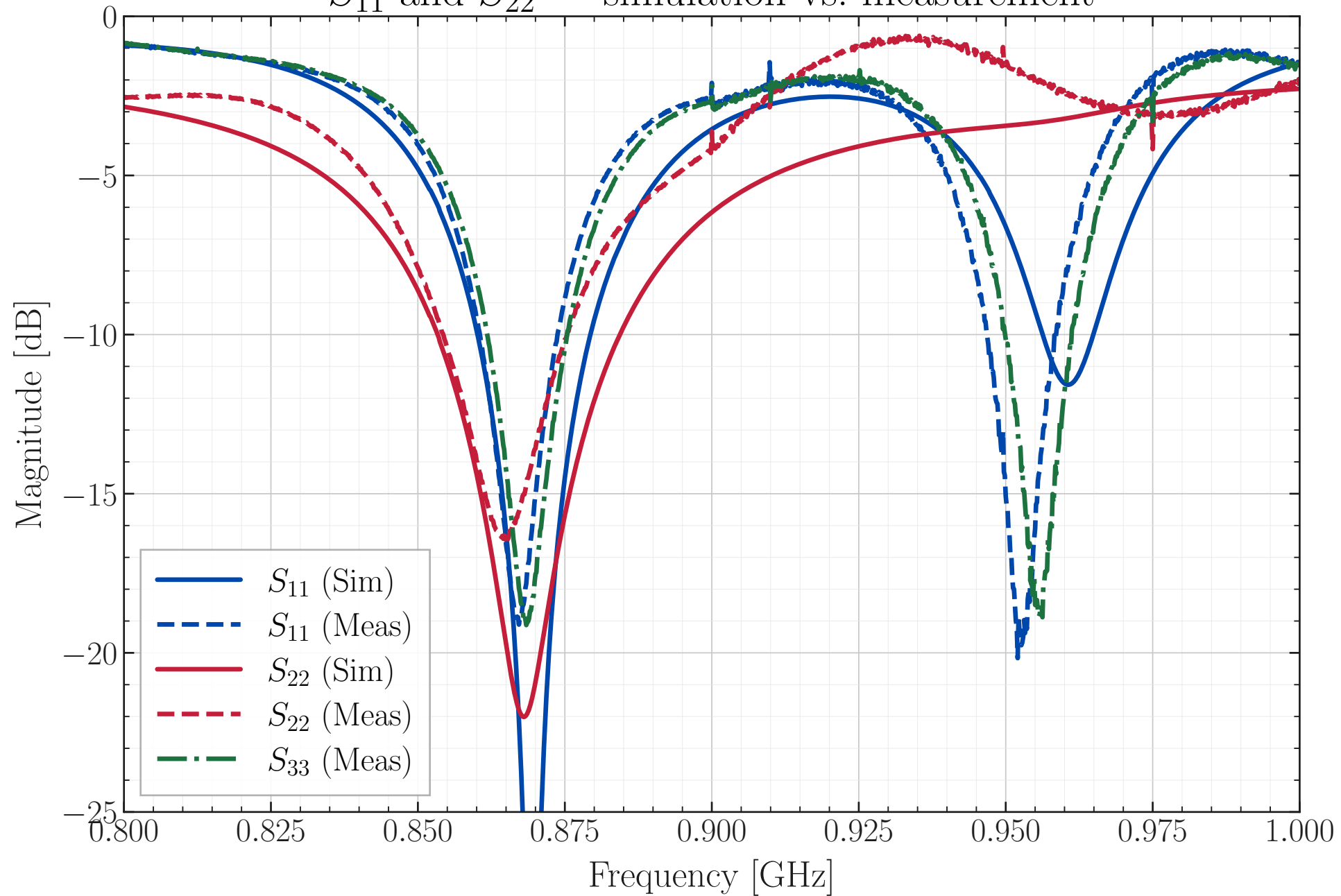
S_{11} and S_{22} — simulation vs. measurement
