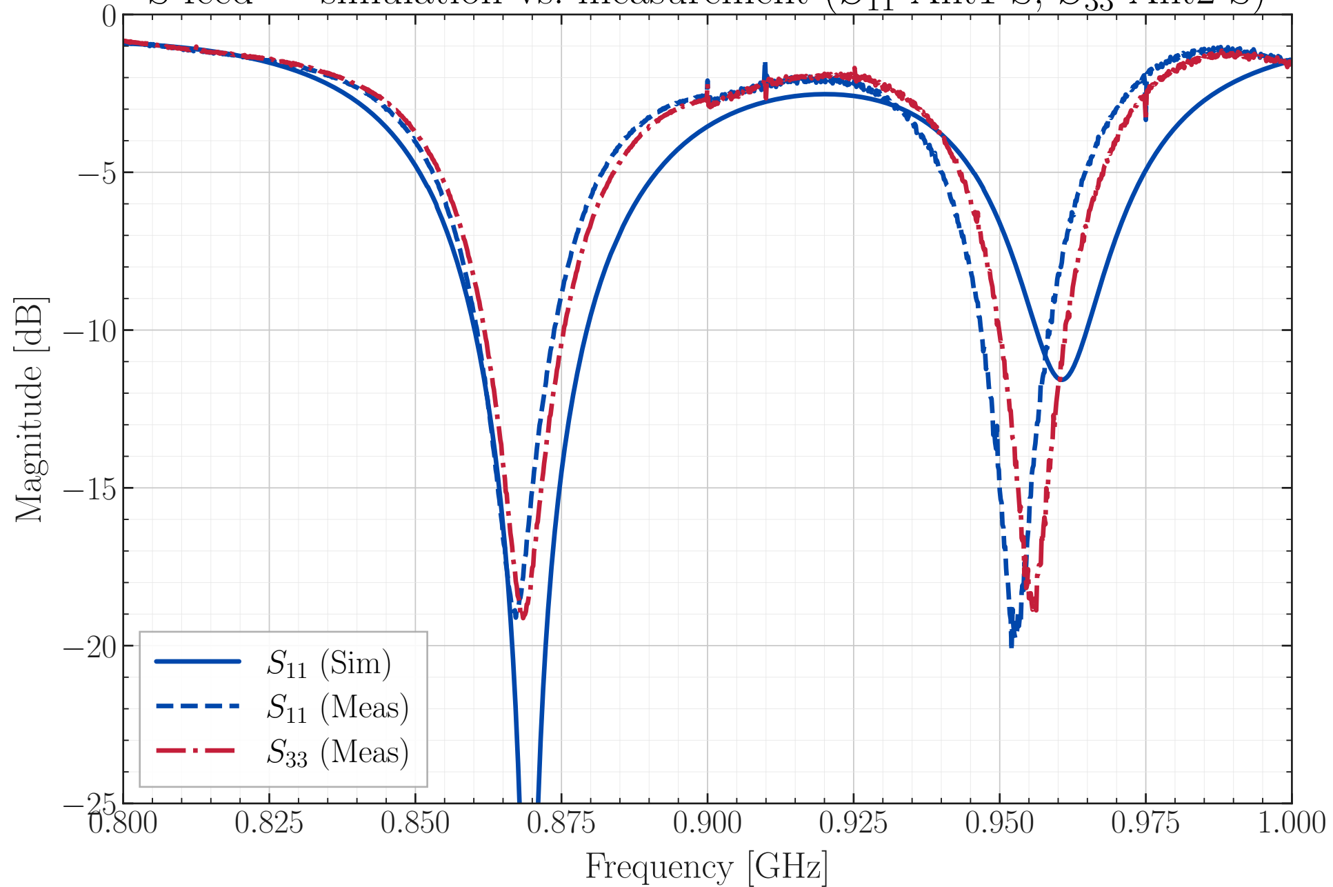
S feed — simulation vs. measurement ( S_{11} Ant1-S, S_{33} Ant2-S)
