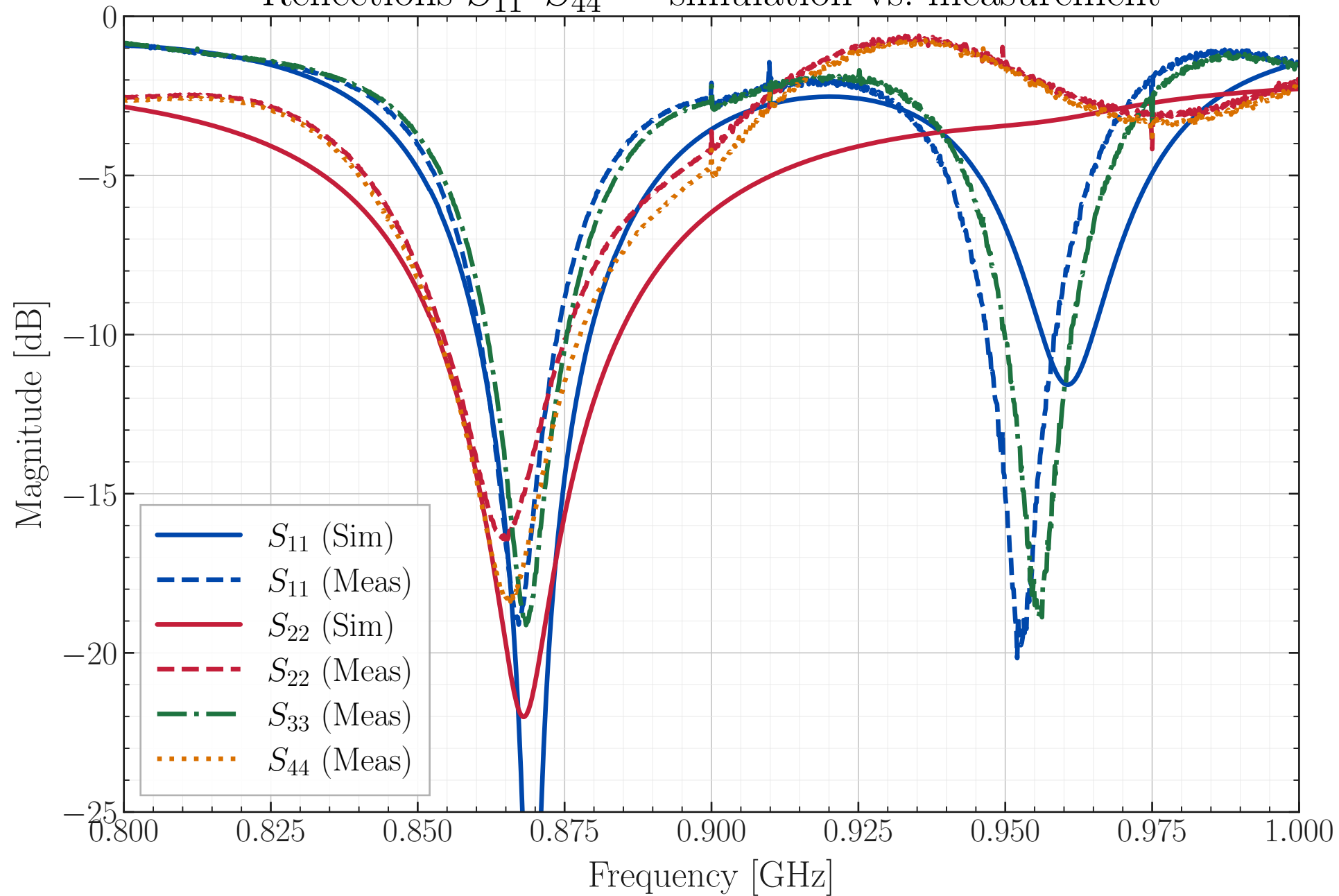
Reflections S_{11} – S_{44} — simulation vs. measurement
