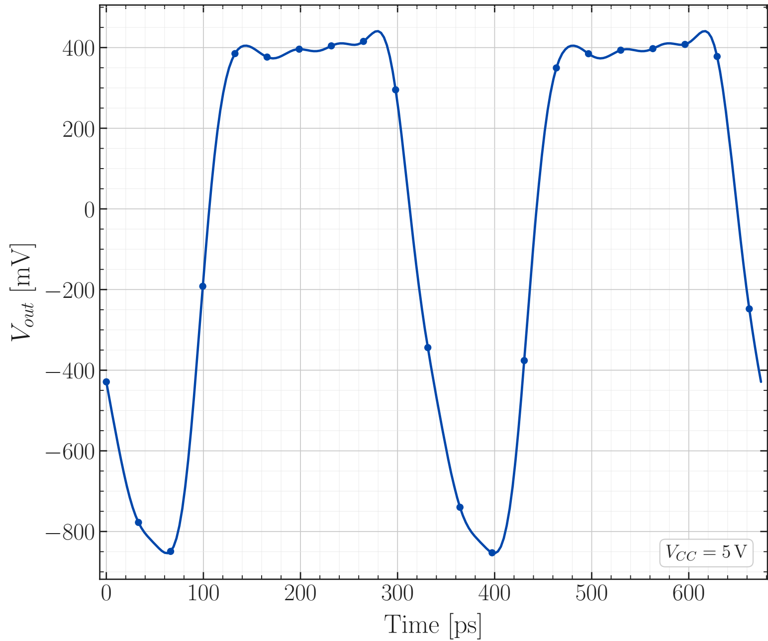
Waveform
