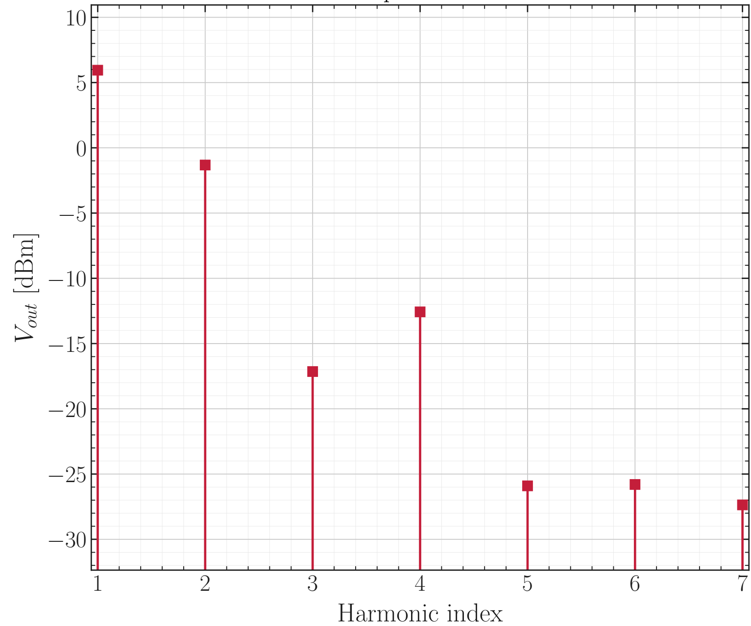
Spectrum
