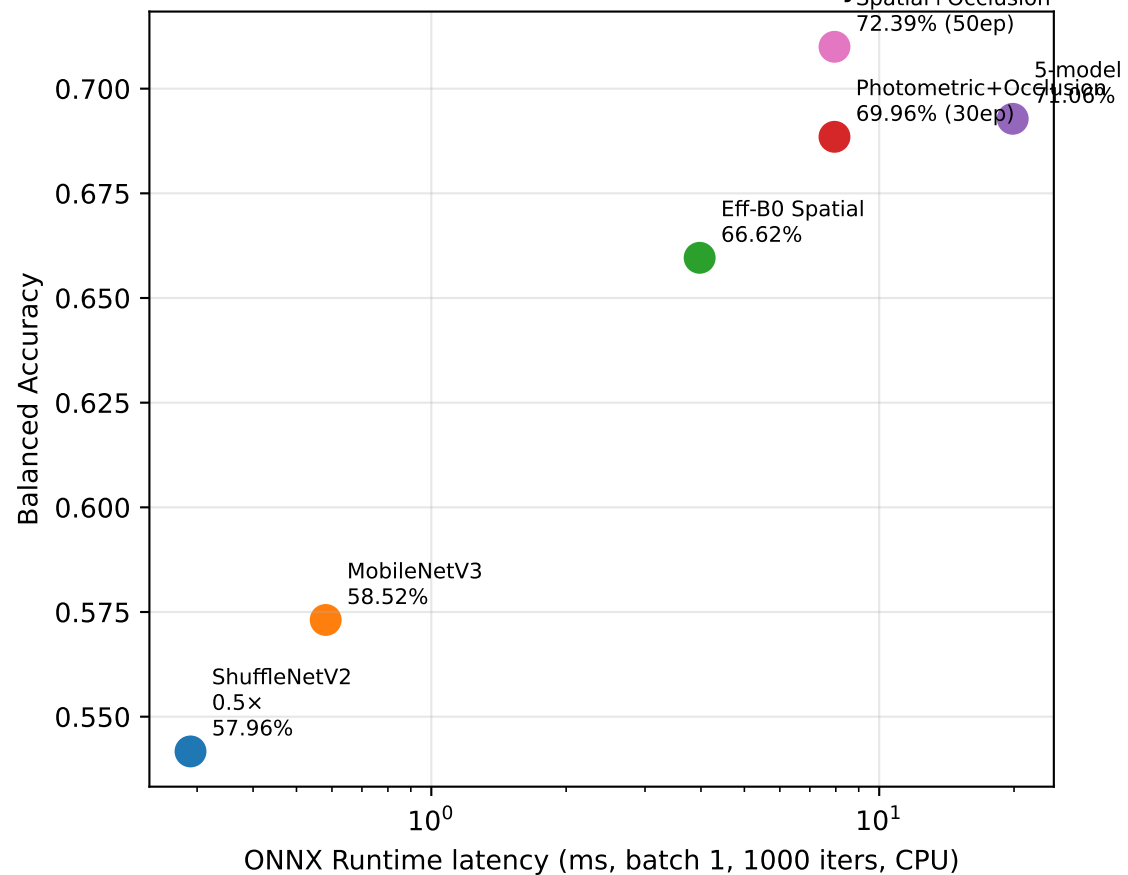
Pareto: Bal Acc vs ONNX latency
