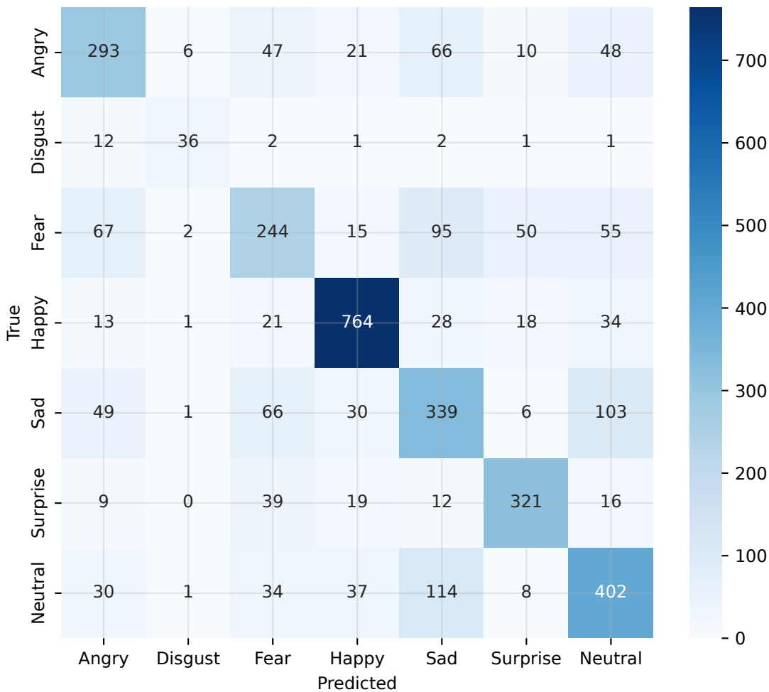
Confusion: V2 (test, acc=0.668)
