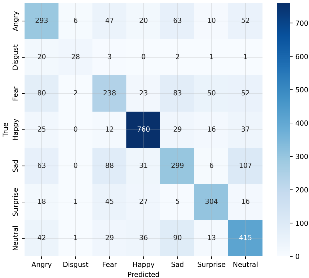
Confusion: V5 (test, acc=0.651)
