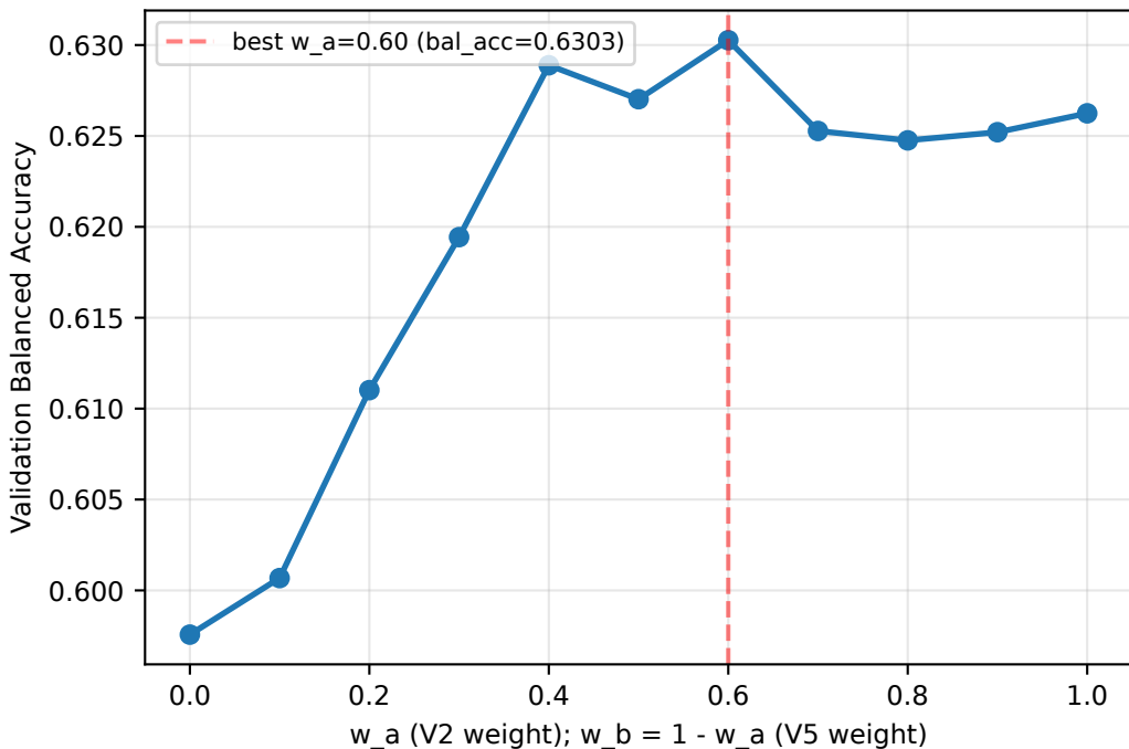
Ensemble weight sensitivity (V2 spatial + V5 mixing)
