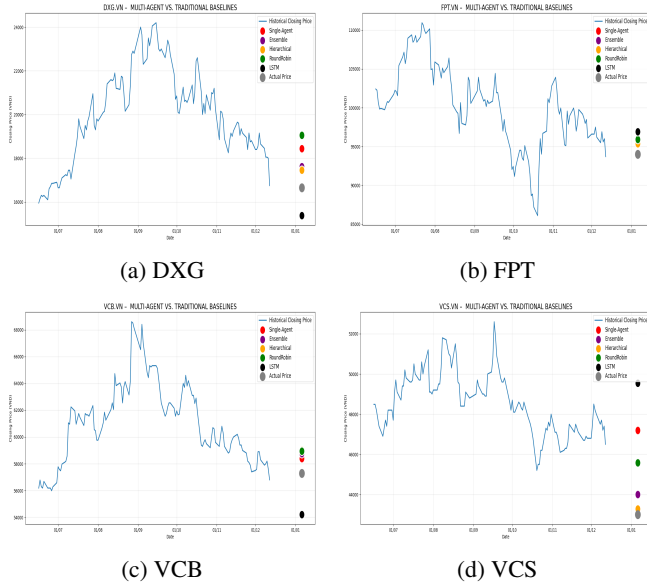
FIGURE 5: Comparative Framework: 14-day Forecasting Results Across Different Approaches
