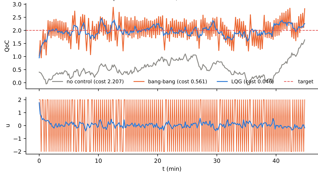
Closed loop on the true model, common random numbers
