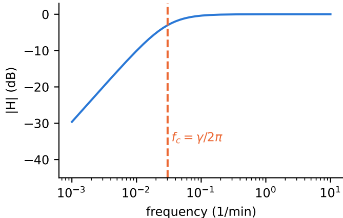
(b) H(s) = s/(s + \gamma) : DC gain = 0
