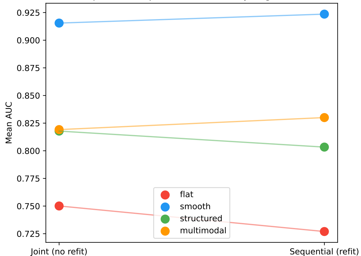
Joint vs Sequential Selection by Regime
