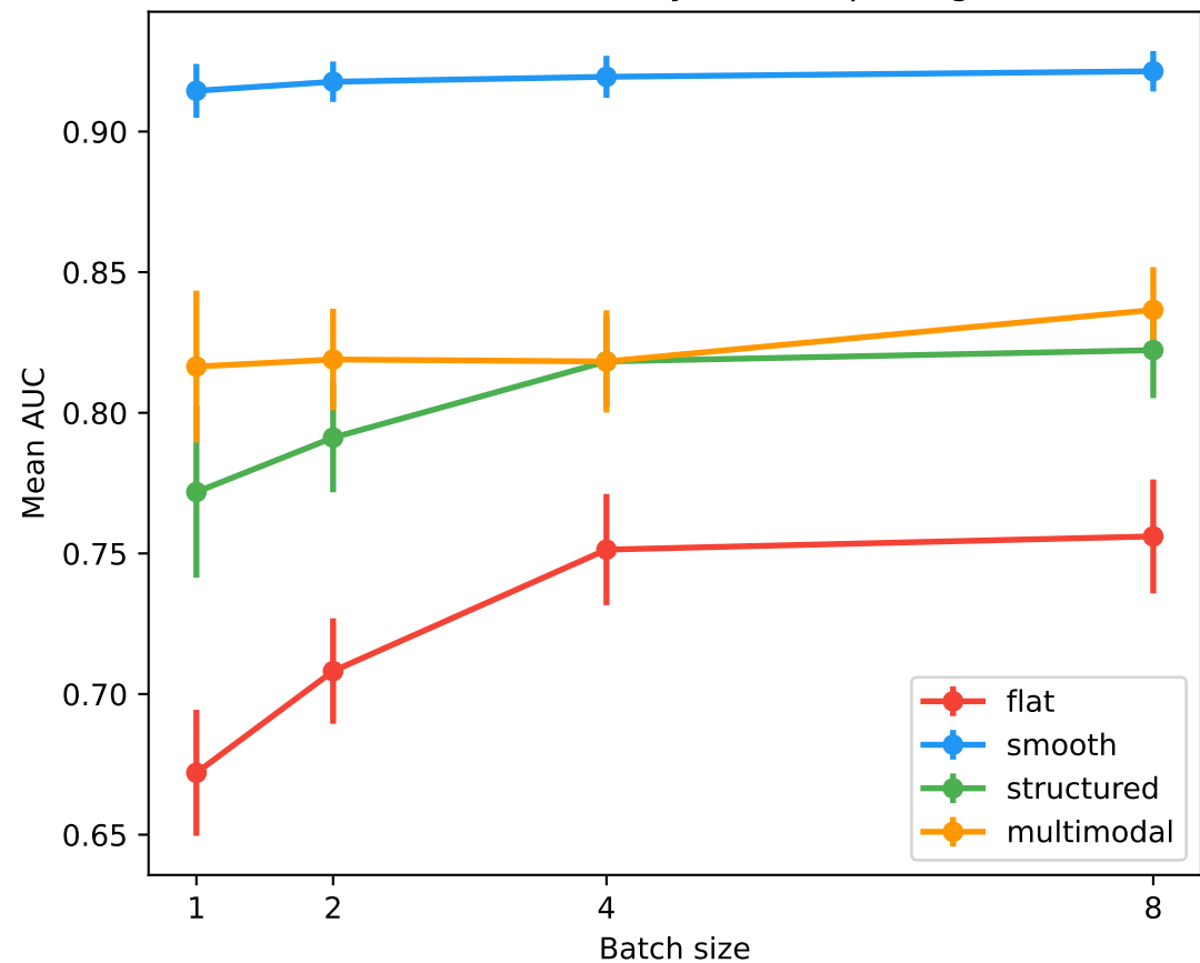
AUC vs Batch Size by Landscape Regime
