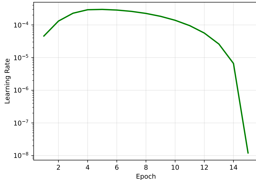
OneCycleLR Schedule
