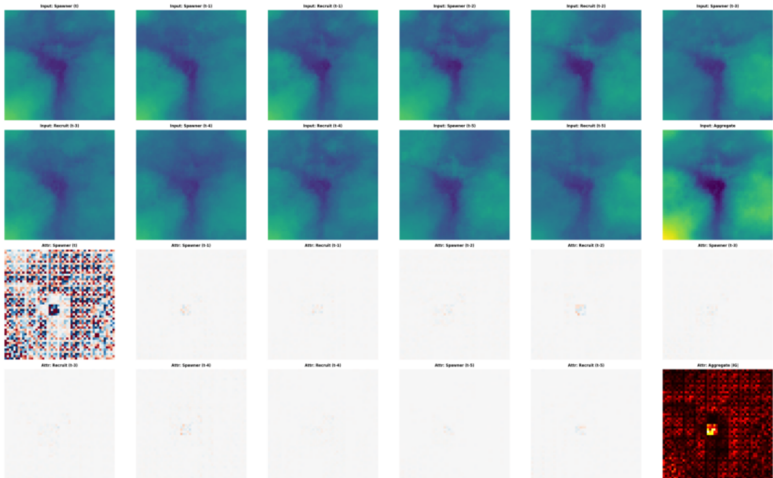
Year 25 — EASY | Tweedie Top: Mean Input (log-space) | Bottom: Attribution (red=+recruit, blue=-recruit)
