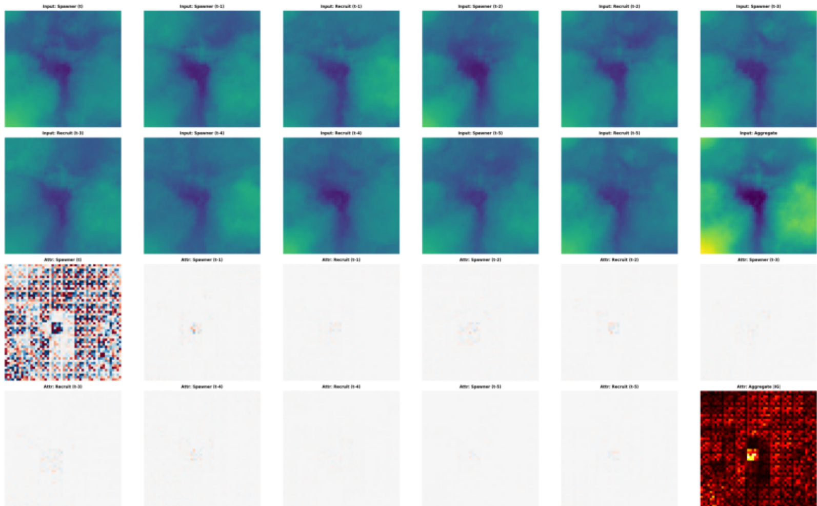
Year 22 — EASY | Tweedie Top: Mean Input (log-space) | Bottom: Attribution (red=+recruit, blue=-recruit)
