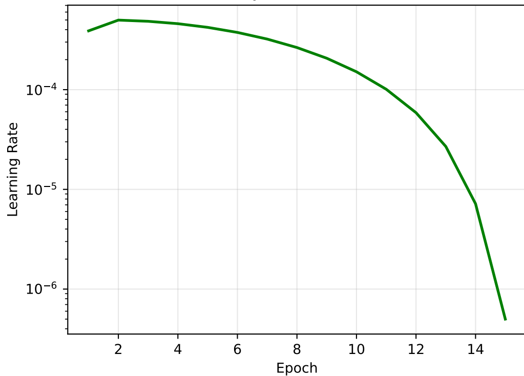
OneCycleLR Schedule
