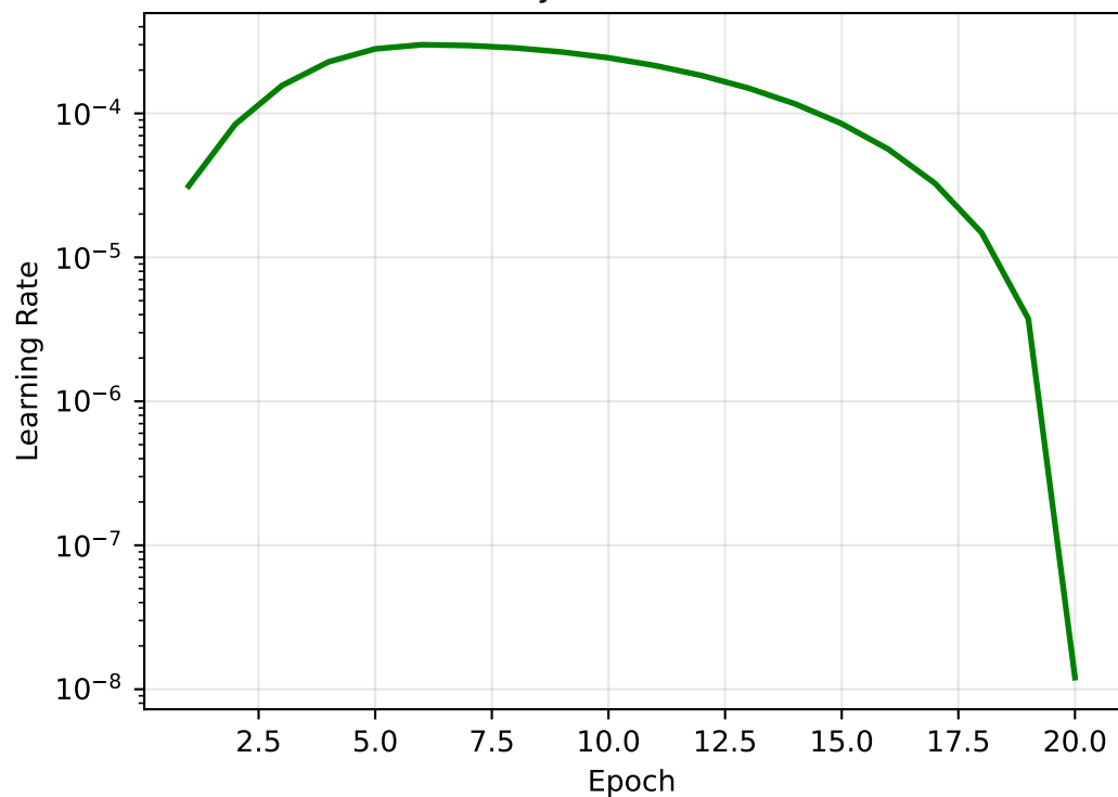
OneCycleLR Schedule
