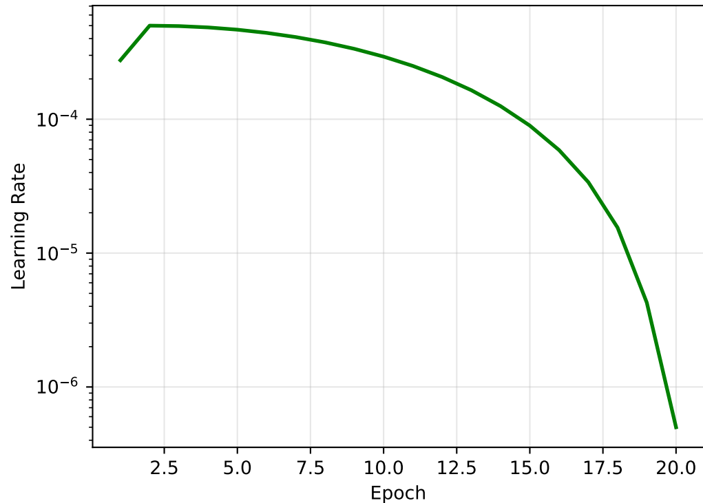
OneCycleLR Schedule
