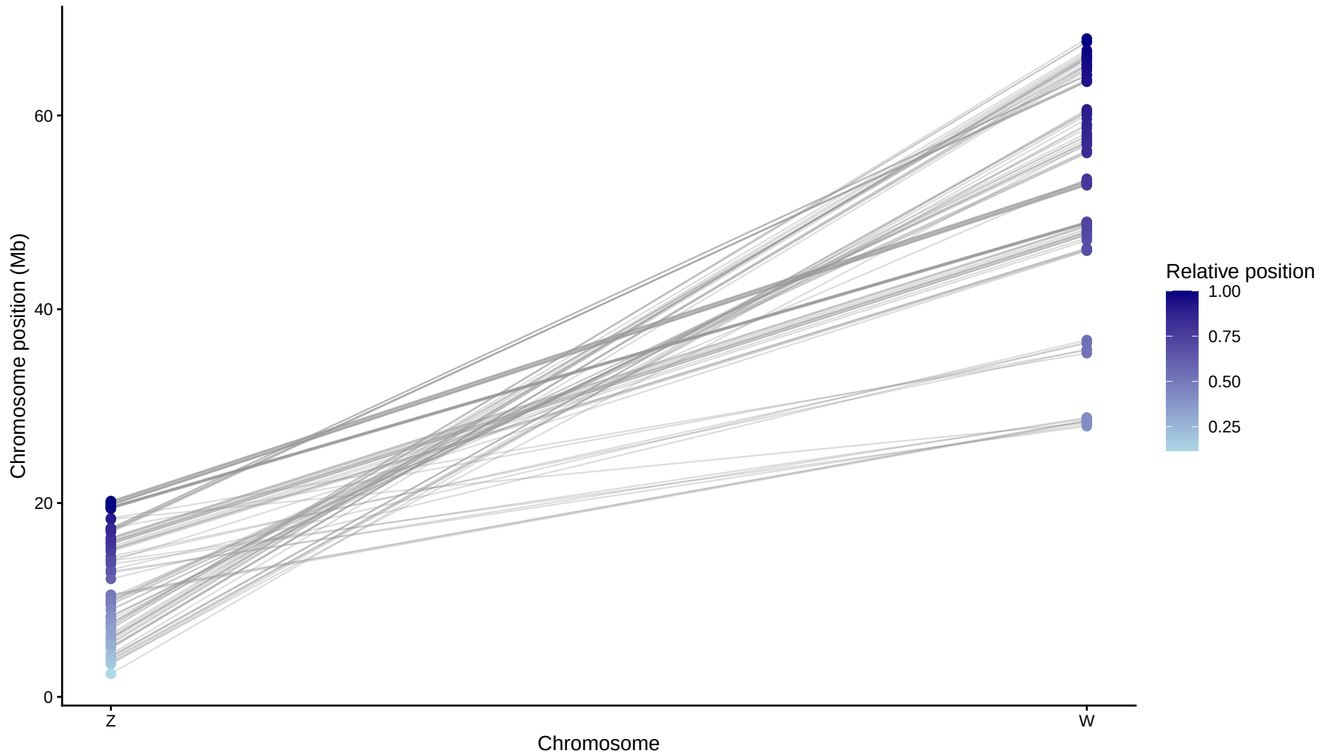
H. suspectum Z and W Gametolog Positions
