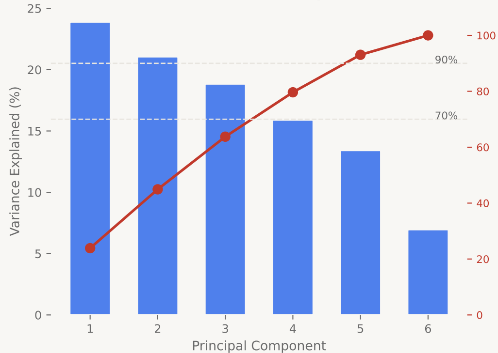
Variance Explained by Each FG Feature Component
