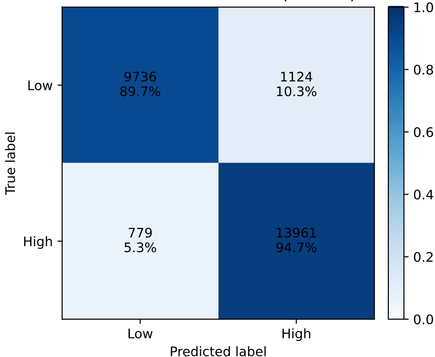
Arousal Confusion Matrix (s01-s32)
