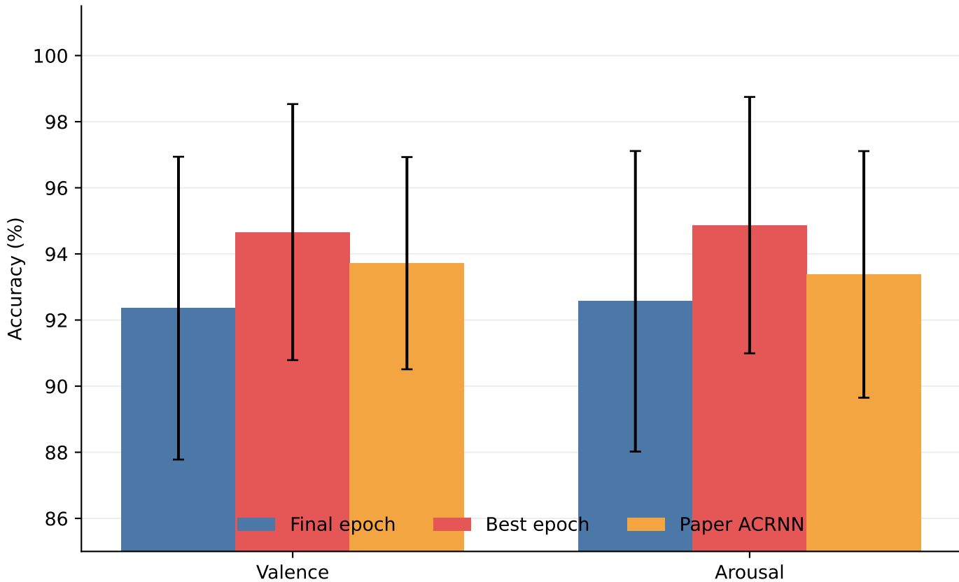
DEAP Overall Accuracy (s01-s32)
