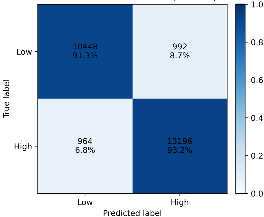
Valence Confusion Matrix (s01-s32)
