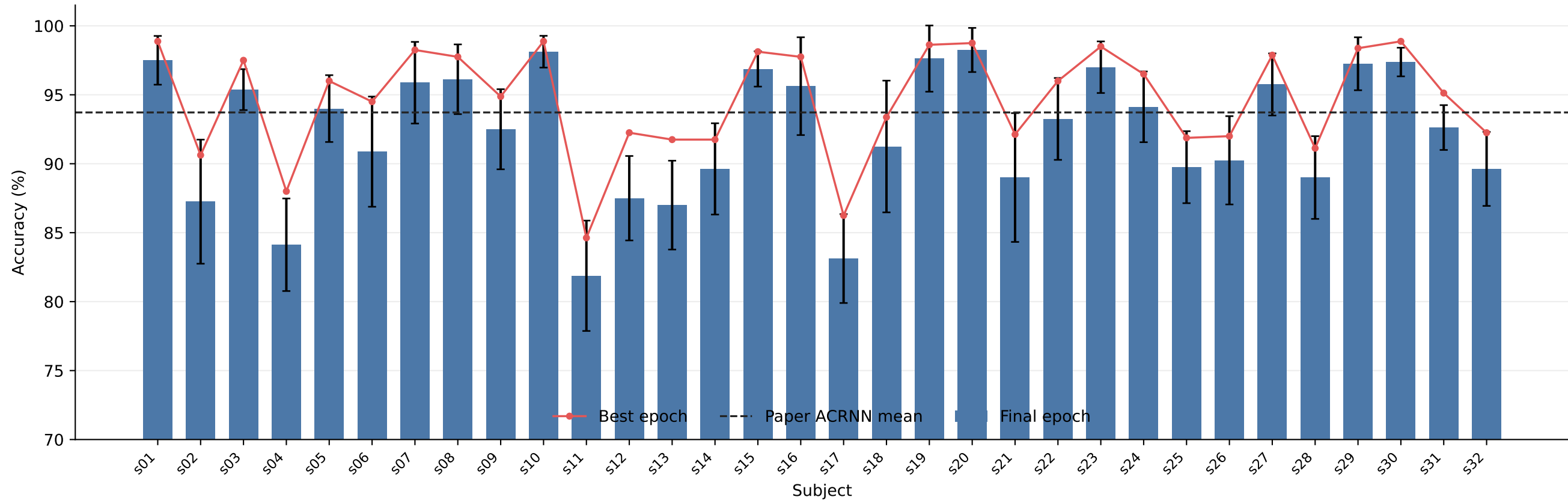
DEAP Valence Classification Accuracy (s01-s32)
