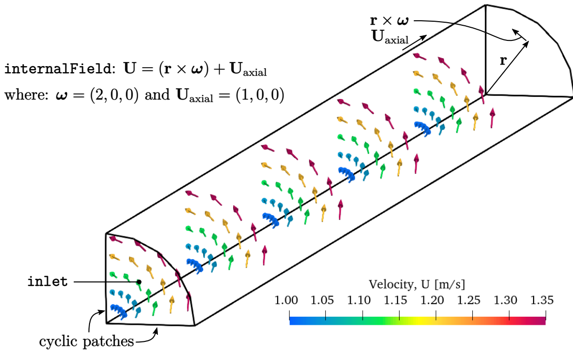
Figure 6.2: Field initialisation with the coded function object.
