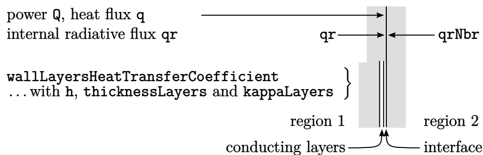
Figure 6.6: The coupledTemperature boundary condition.
