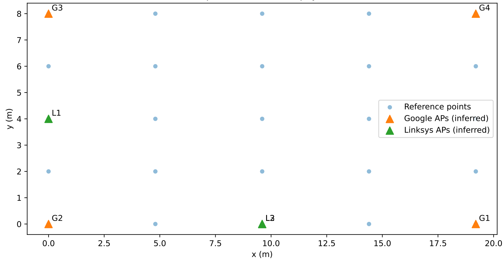
EETAC reference points and inferred physical AP locations
