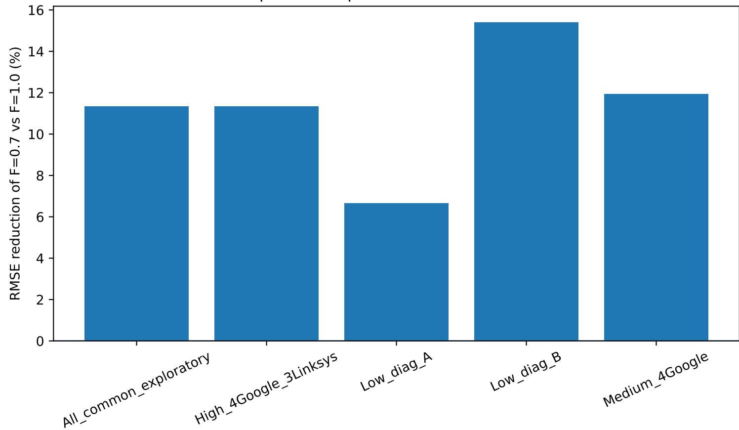
Subspace RF improvement: stratified row cv
