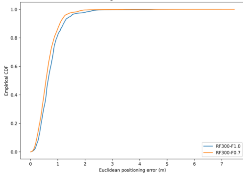
Building: localization-error CDF
