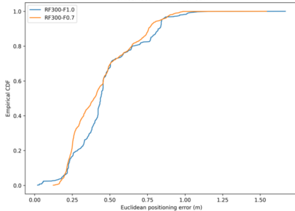
Office: localization-error CDF
