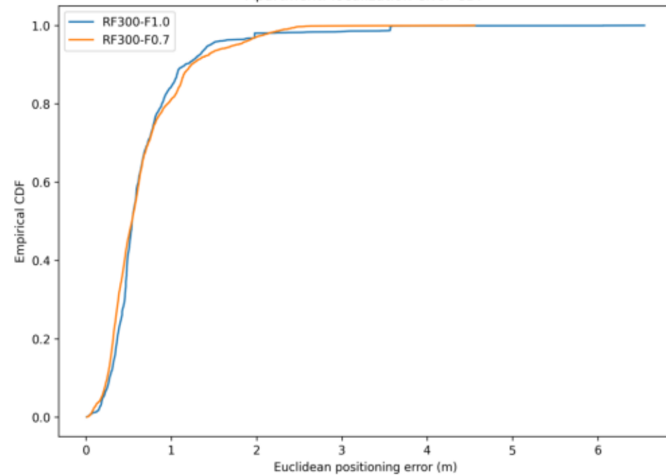
Apartment: localization-error CDF
