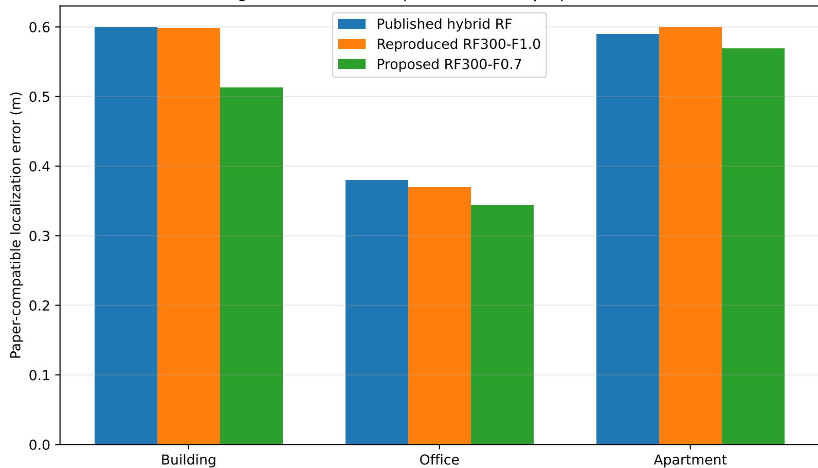
Original benchmark: reproduction and proposed model
