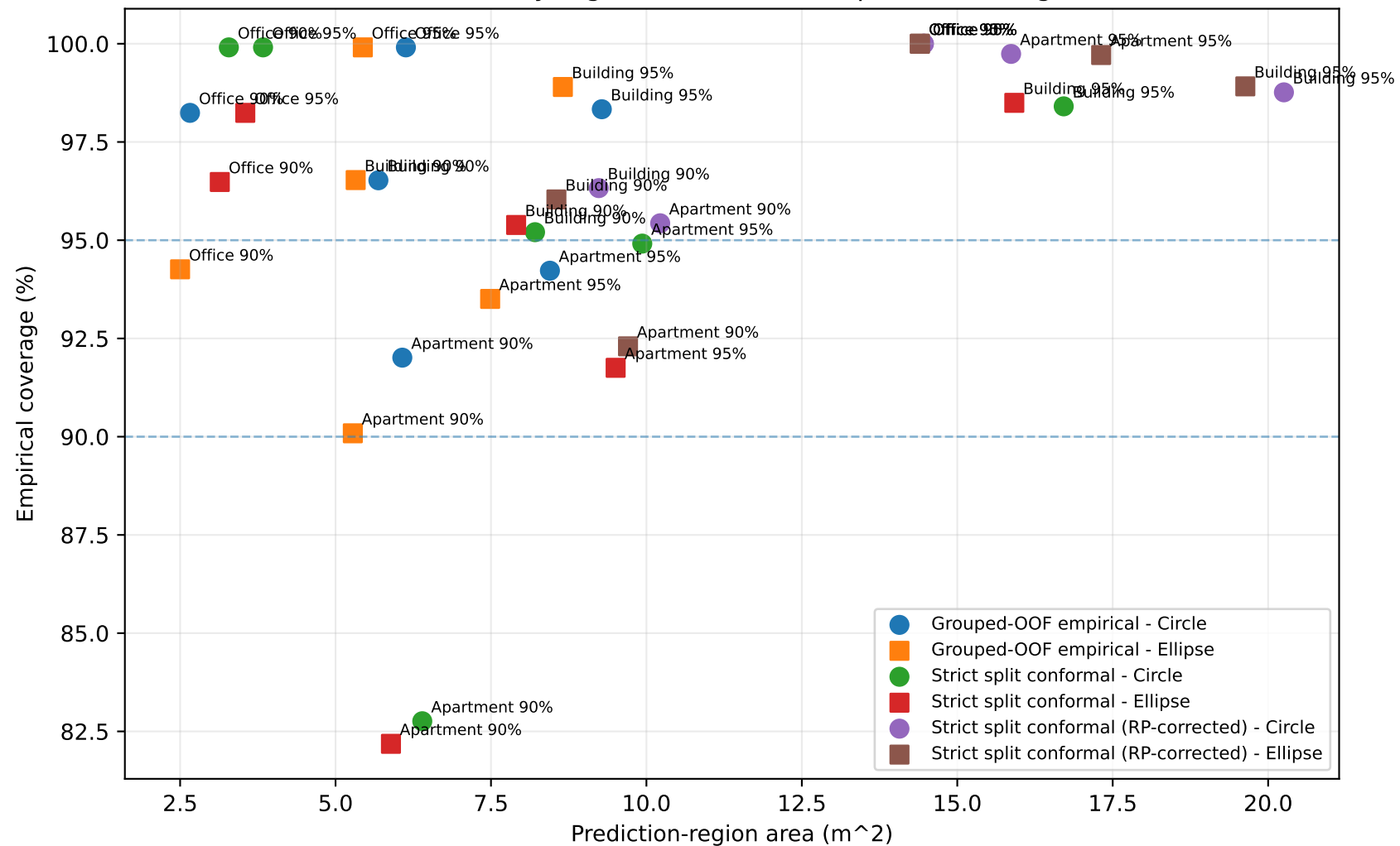
Uncertainty-region area versus empirical coverage
