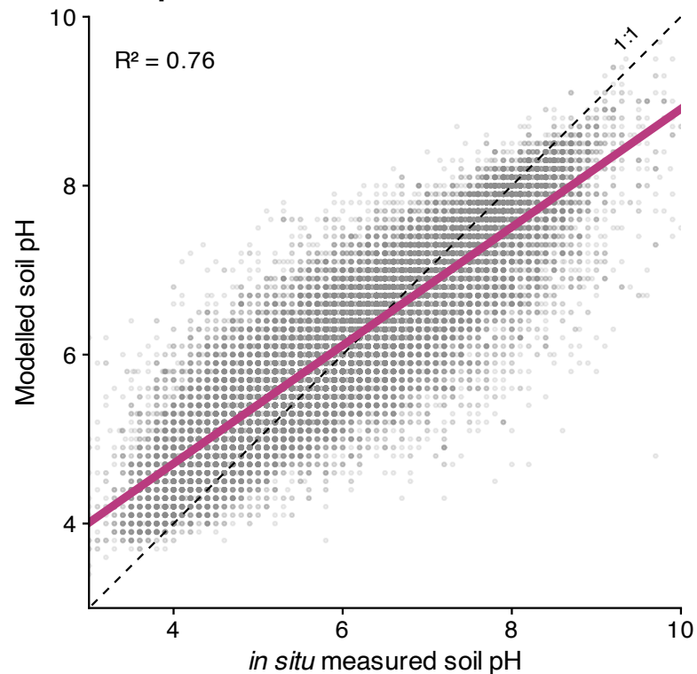
Soil pH
