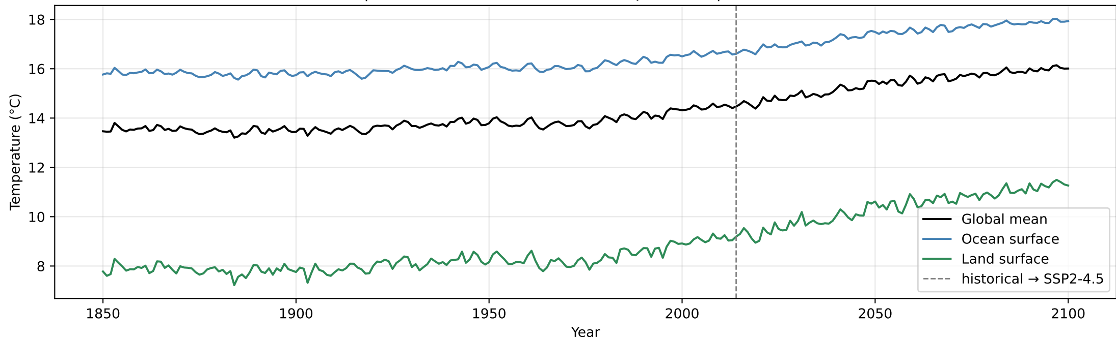
MPI-ESM1-2-LR | Annual Mean Near-Surface Temperature | Historical + SSP2-4.5 (r1)
