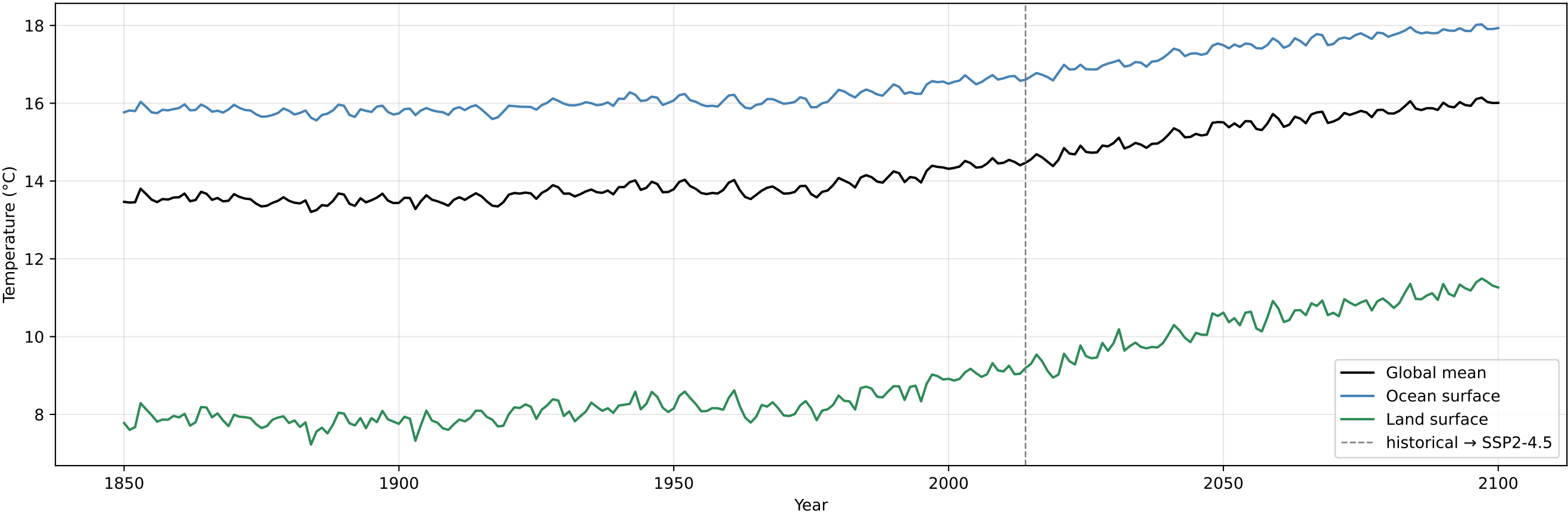
MPI-ESM1-2-LR | Annual Mean Near-Surface Temperature | Historical + SSP2-4.5 (r1)
