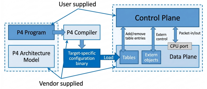
Fig. 7. P4 workflow.
