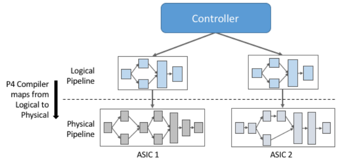
Fig. 5. A logical pipeline mapped by the P4 compiler onto the physical pipelines of two different ASICs. Adapted from [1].
