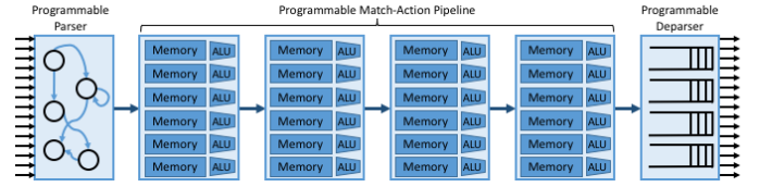
Fig. 5. Abstract forwarding pipeline that model how most data plane devices are forwarding packet. Adapted from [1].
