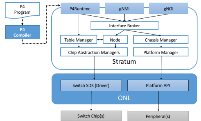
Fig. 9. "Thin" Switch OS architecture that is designed for vendor-agnostic. Adapted from [1].
