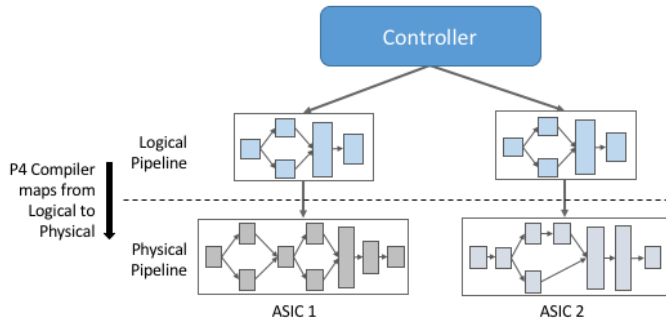
Fig. 6. A logical pipeline mapped by the P4 compiler onto the physical pipelines of two different ASICs. Adapted from [1].
