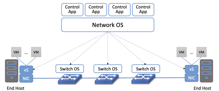
Fig. 3. End-End network view of SDN architecture. Adapted from [1].
