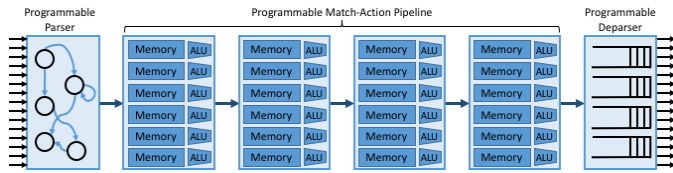
Fig. 4. Abstract forwarding pipeline that model how most data plane devices are forwarding packet. Adapted from [1].
