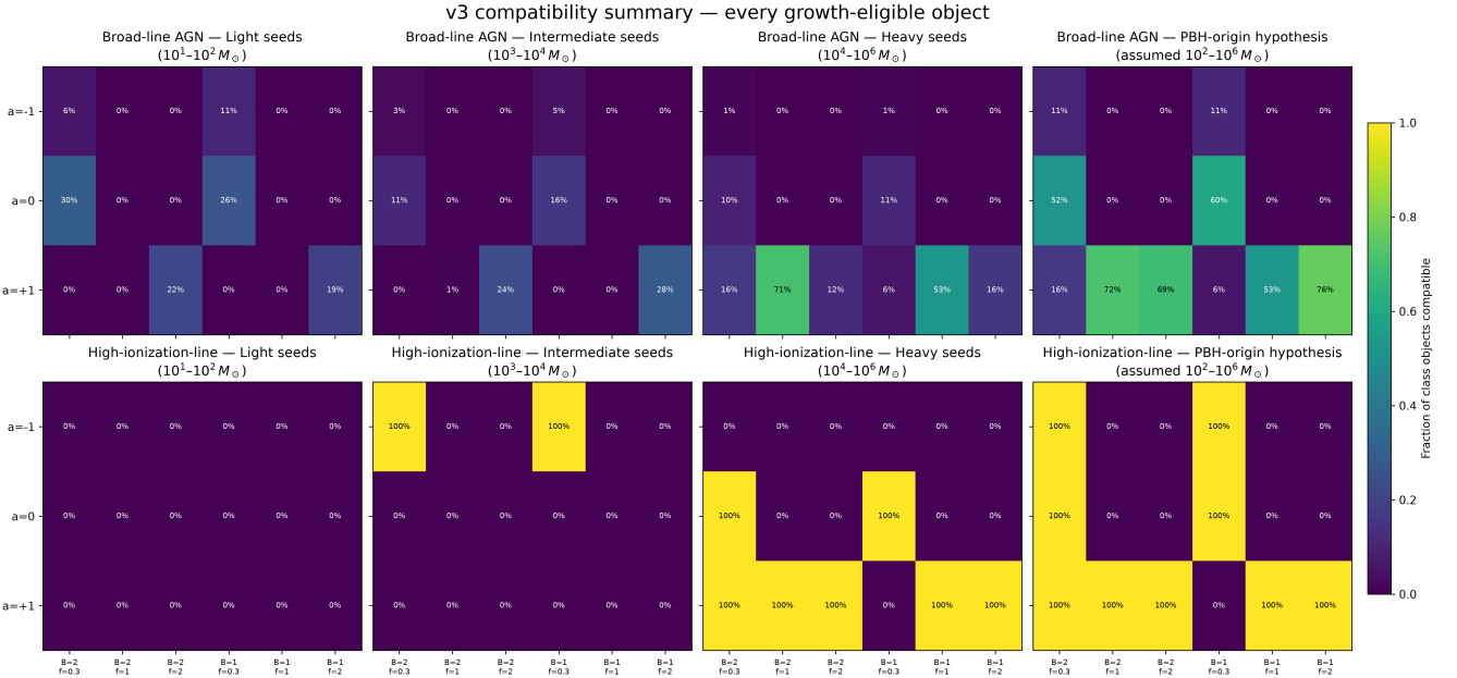
Figure 4: Compatibility summary using every one of the 153 growth-computable objects. Panels retain object class and seed family while spanning spin, merger boost, and average accretion rate. Percentages are descriptive within-class fractions, not pooled demographic estimates. The complete object-by-object matrix, including all 21 unavailable objects, is included in the supplement.
