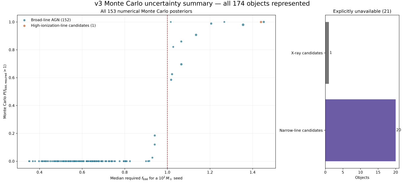
Figure 5: Complete Monte Carlo uncertainty summary. Every one of the 153 numerical posteriors is plotted; point size encodes the 16th–84th percentile width. The adjacent accounting panel retains all 21 catalogue-only objects. The full supplement atlas gives every object label and interval.
